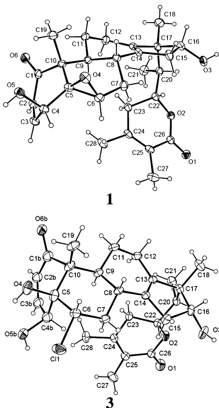
Figure 1. Computer-generated ORTEP diagrams of compounds 1 and 3 .
